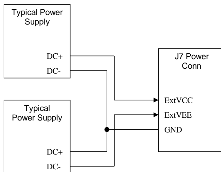
Figure 3-9: GX5964/GX5964A Typical Power Connection Diagram
