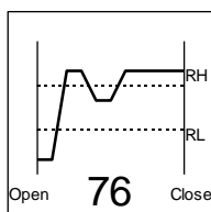
Rising Edge Glitch – Signal starts below RL, crosses RL once, crosses RH one or more times and ends above RH.
