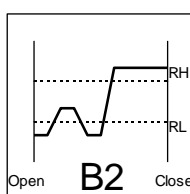
Low Glitch Rising Edge - Signal starts below RL, crosses the RL one or more times, crosses RH once and ends above RH.
