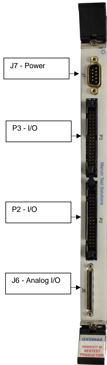
Figure 3-7: GX5964A Front Panel Connectors
