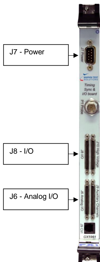
Figure 3-5: GX5961 Front Panel Connectors
