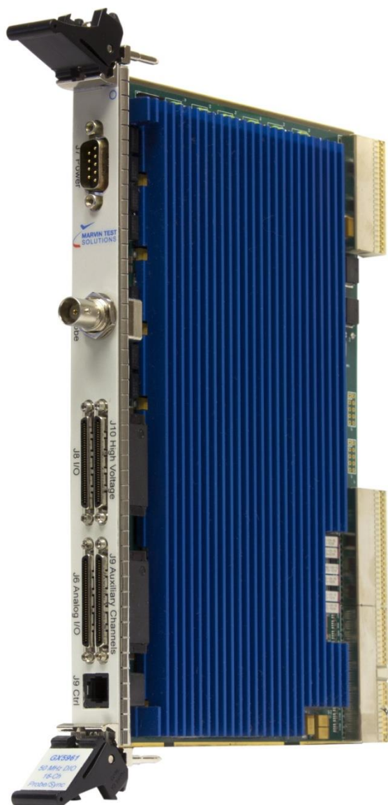
Figure 2-1: GX5961 Board
