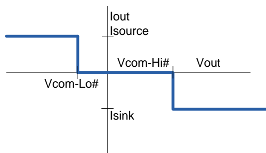
Figure 4-17: GX5960 Input Load Current Voltage Clamps
