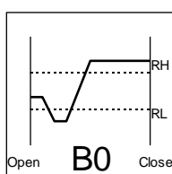
Middle Rising Edge - Signal starts between RL and RH, crosses the RL one or more times, crosses RH once and ends above RH.
