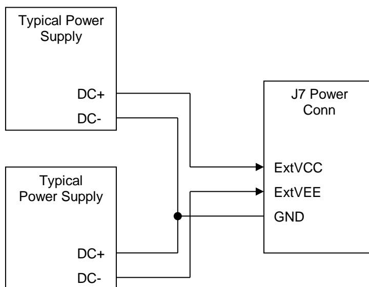
Figure 3-8: GX5961 Typical Power Connection Diagram
