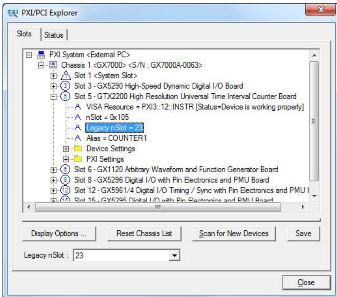
Figure 3-1: PXI/PCI Explorer
